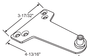
19-210 Parallel Bracket
