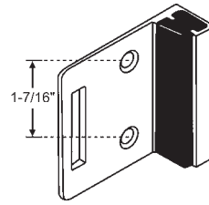
91-135 Inswing for Slide Latch
