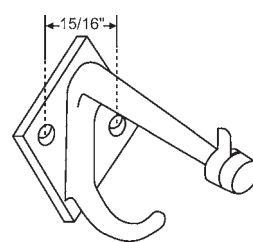
91-255 1/4" Hole Diameter
