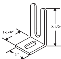
91-22 Floor Bracket
