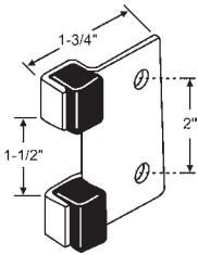
91-88 Inswing/Outswing Strike SANYMETAL
