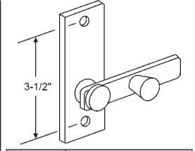
91-292 For 1" Steel Door
