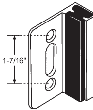
91-140 Inswing/Outswing for Concealed Latch
