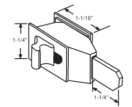
900-18069 With Red and Green Indicator. For 1" Steel Door
