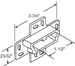
45-23 Drawer Mounting Bracket
