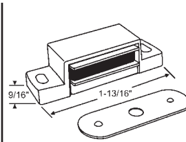
45-194 Brown Plastic Magnetic Cabinet Door Catch with Flat Plate
