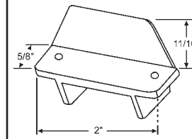
45-10 Drawer Guide
