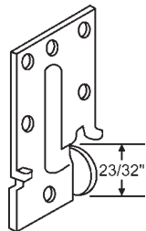
900-17778 Roller Bracket No Longer Available. Use: 900-17778NS
