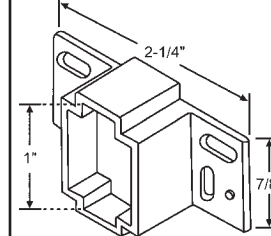
45-16 Drawer Bracket
