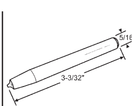
59-81 Rivet Installation Tool
