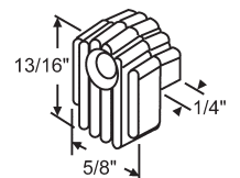
900-9137 Ribbed Mirror Clip without Screws
